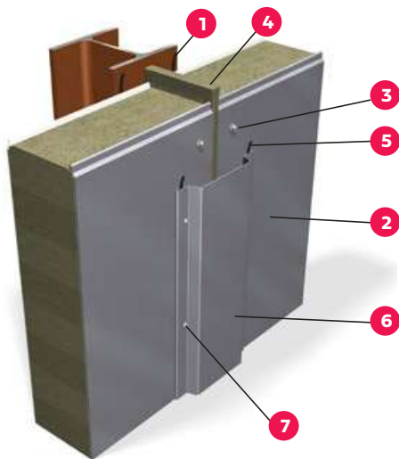
Figure 19. Fastening of Paroc Panel System panels using penetrating panel fixings.
