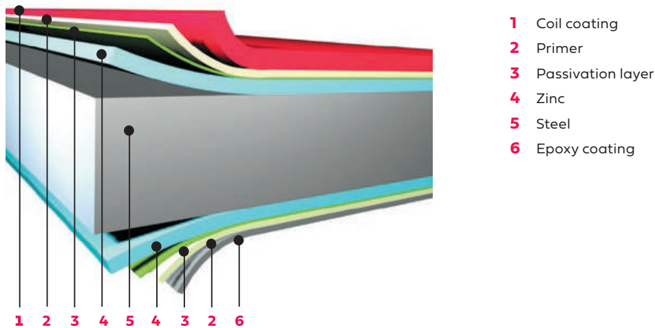
Figure 2. Facing structure of PPS panels.
