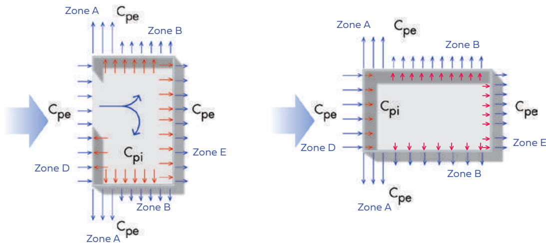
Figure 7. Pressure coefficients.
